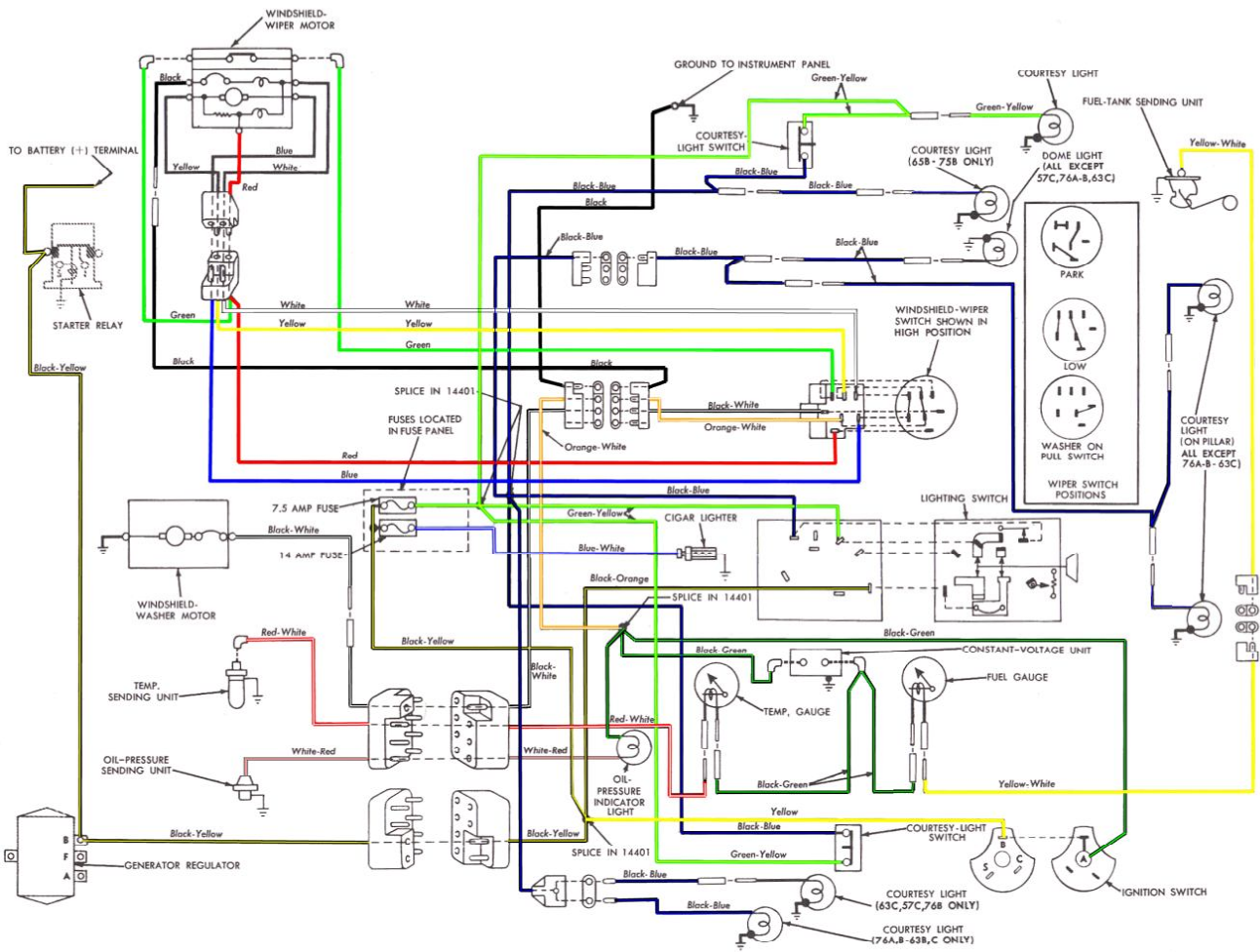
FIG. 3—Interior Lighting, Windshield Wiper, Gauges, and Heater Schematic—Ford
